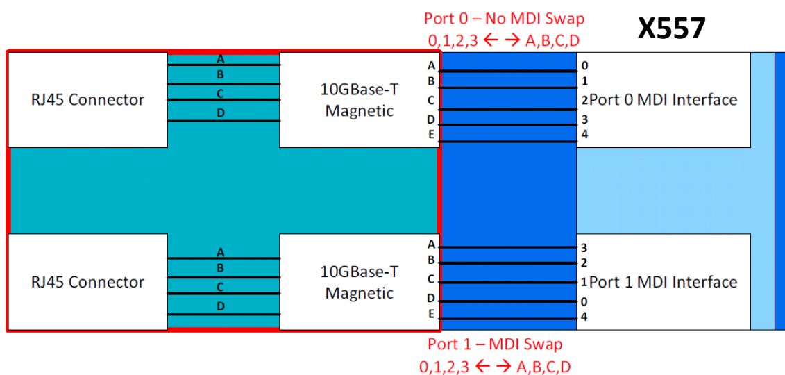
Figure 9-6 PHY AFE_LINE Lane Swap Configuration
